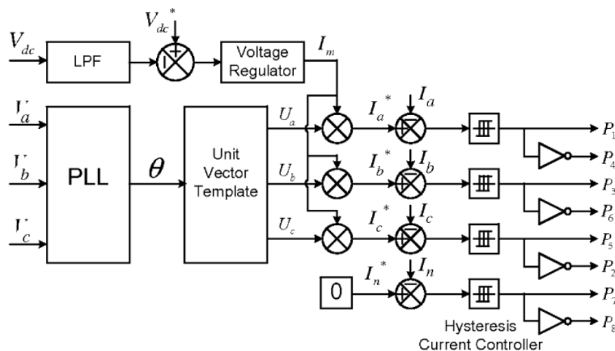
Fig.3. Block diagram representation of grid-interfacing inverter control.
