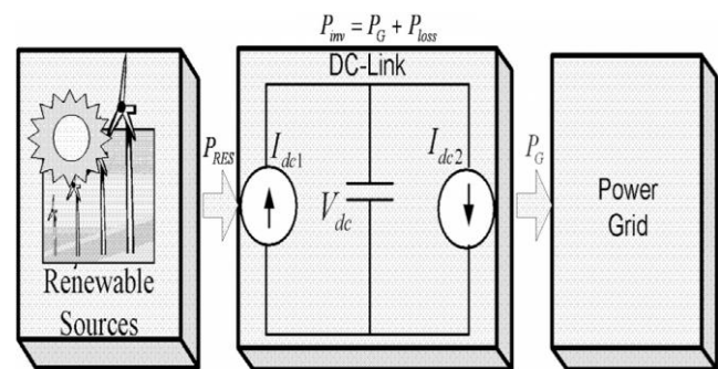
Fig.2.DC-Link equivalent diagram.
