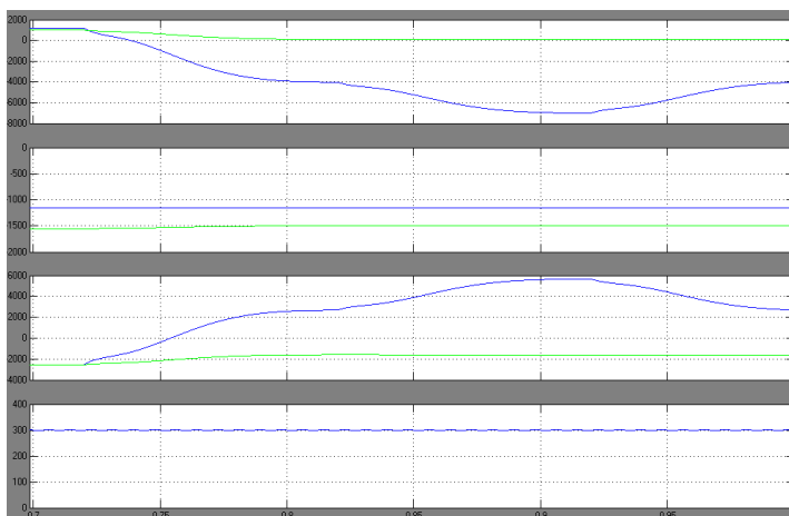
Fig.6. Simulation results: y-axis- (a) PQ-Grid, (b) PQ-Load, (c) PQ-Inverter, (d) dc-link voltage, x-axis time sec.
