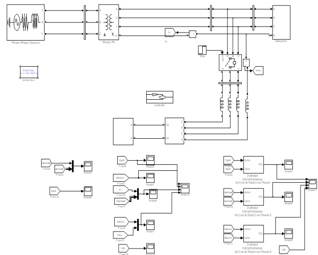
Fig 4. simulink modal of proposed system.
