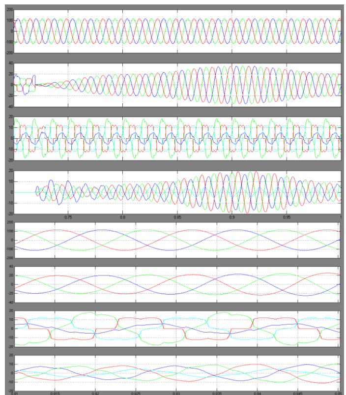
Fig. 5. Simulation results: y-axis - (a) Grid voltages, (b) Grid Currents (c) Unbalanced load currents, (d) Inverter Currents, x-axis-time in sec.
